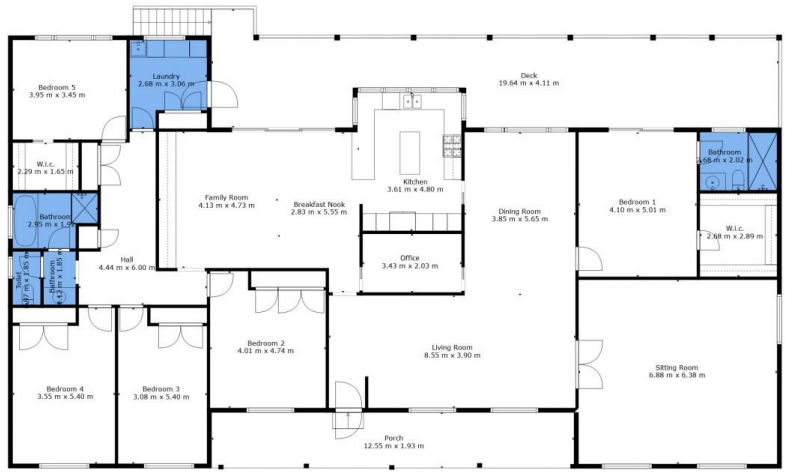
Floor 2
